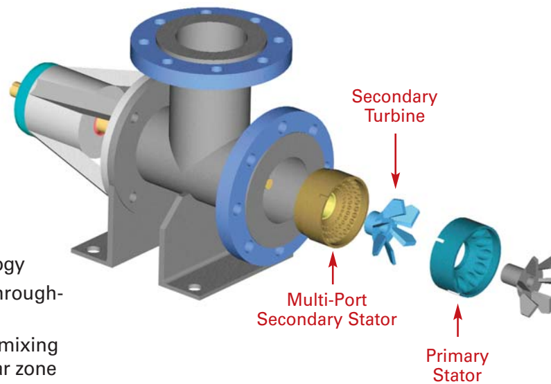
Standard Tandem Shear Configuration
